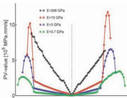
Figure 7—PV values found for a steel pinion meshing with gears of various materials.
