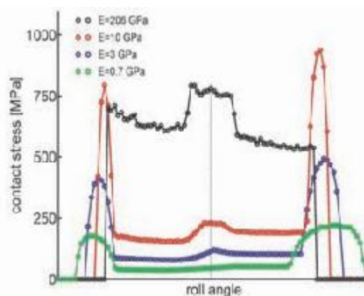
Figure 6—(Hertzian) contact stress as a function of the roll angle for a steel pinion meshing with a gear of various materials.
