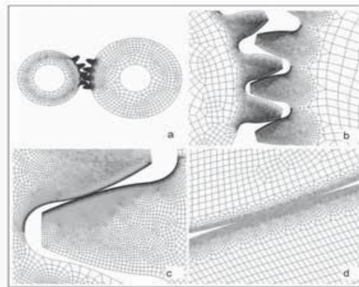
Figure 1—Details of the FE mesh. An overview of the complete model is shown in figure a, while zooming in on the refined mesh in the contact area from figures b to d.
