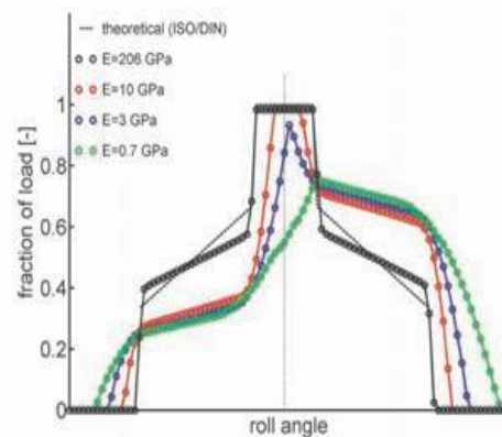
Figure 2—Load sharing between teeth of a steel pinion and a steel gear (black circles), a glass fiber (GF)-reinforced plastic gear (red circles), an unfilled plastic gear (blue circles) and an unfilled gear at elevated temperature (green circles). The dashed black line represents the theory (ISO 6336) and the dotted black line indicates the pitch point.
