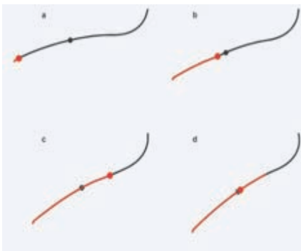
Figure 8—Kinematics of two meshing tooth flanks (only gear flank is drawn). The solid black line represents the tooth flank of the gear, the black dot represents the pitch point, the red dot represents the moving contact point and the solid red line represents the part of the flank that has already been in contact.
