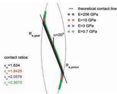
Figure 4—Contact path during meshing of a steel pinion with a gear of various materials.
